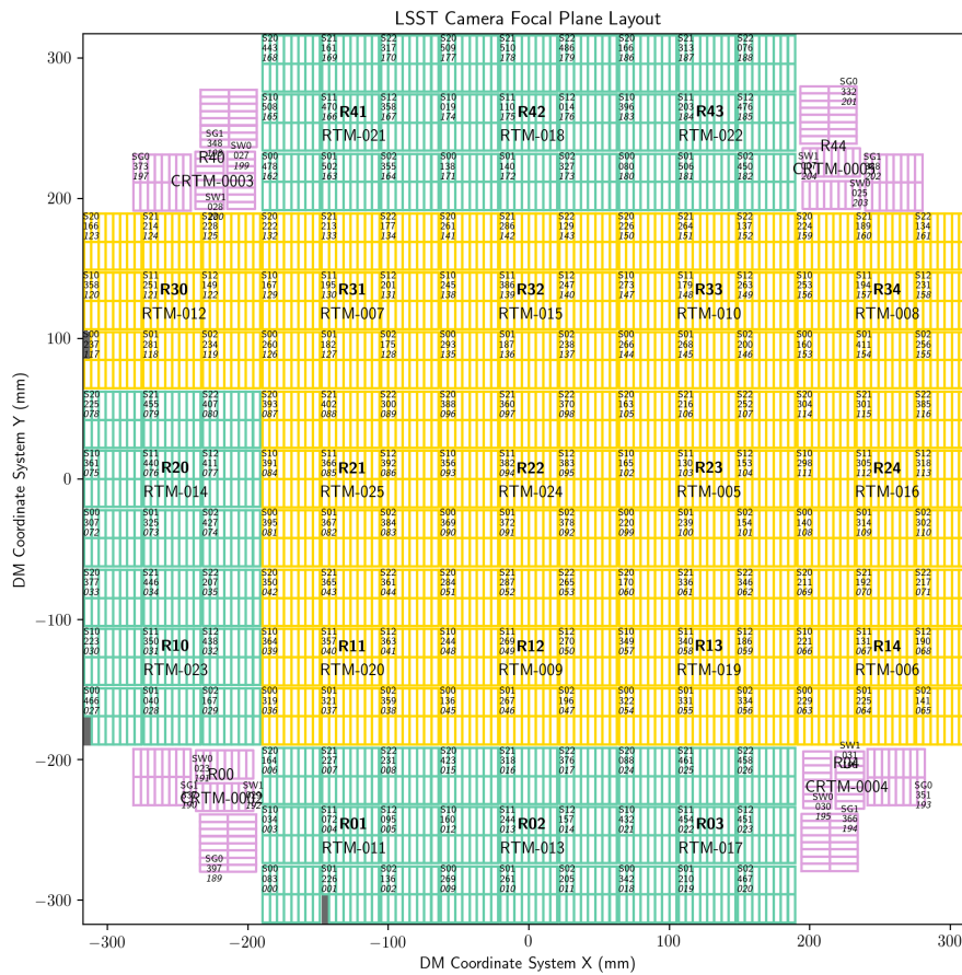
FIGURE 1: Focal Plane map of all the CCDs on the Rubin Observatory LSST Camera (see also CTN-001 for more detail). Yellow and green areas show CCDs manufactured by two different vendors. Our dataset for task 1 comes from a CCD on the third raft at the bottom right corner.
