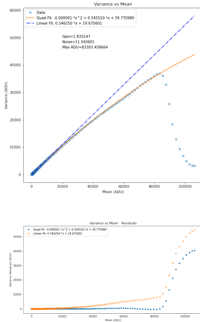
FIGURE 2: Top: Quadratic and linear fit made with np.polyfit . Quadratic fit made using data points up to maximum variance. Linear fit made with points with \mu < 10000 ADU. Bottom: Residuals for both fits.
